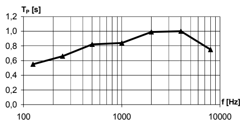
Fig. 2 RT of the measured auditory room
